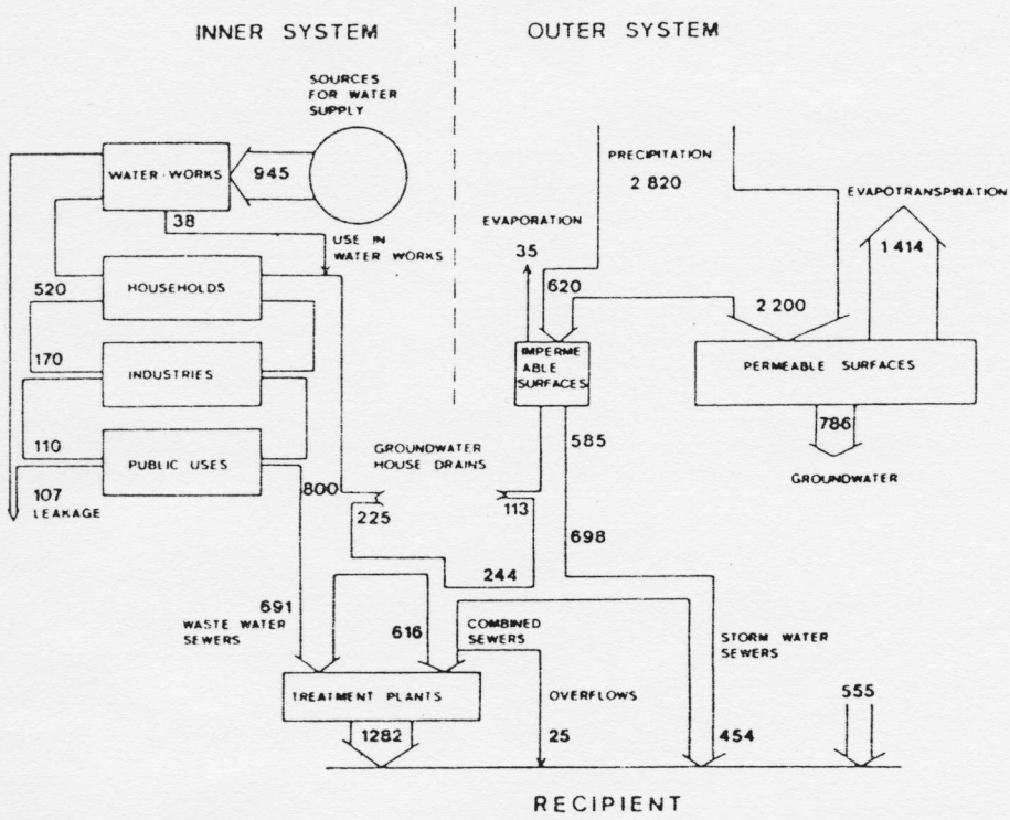
Fig. 2.6. General urban area water budget for Sweden ( \times 10^4 \text{ m}^3/\text{year} ) (Carlsson and Falk, 1977).
